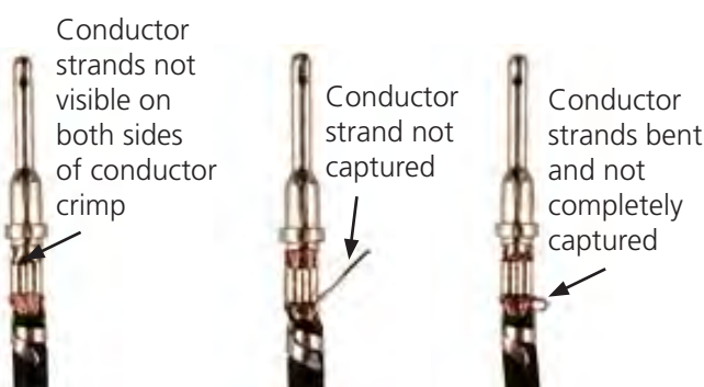
Unacceptable Crimps
