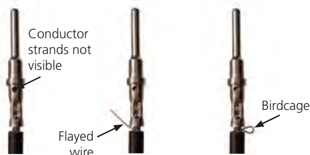
Unacceptable Crimps
