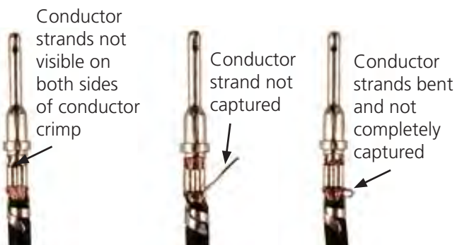
Unacceptable Crimps
